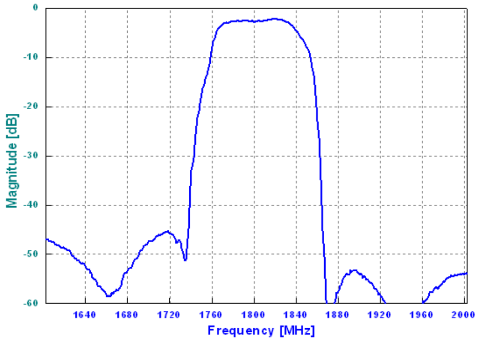
Frequency Response
